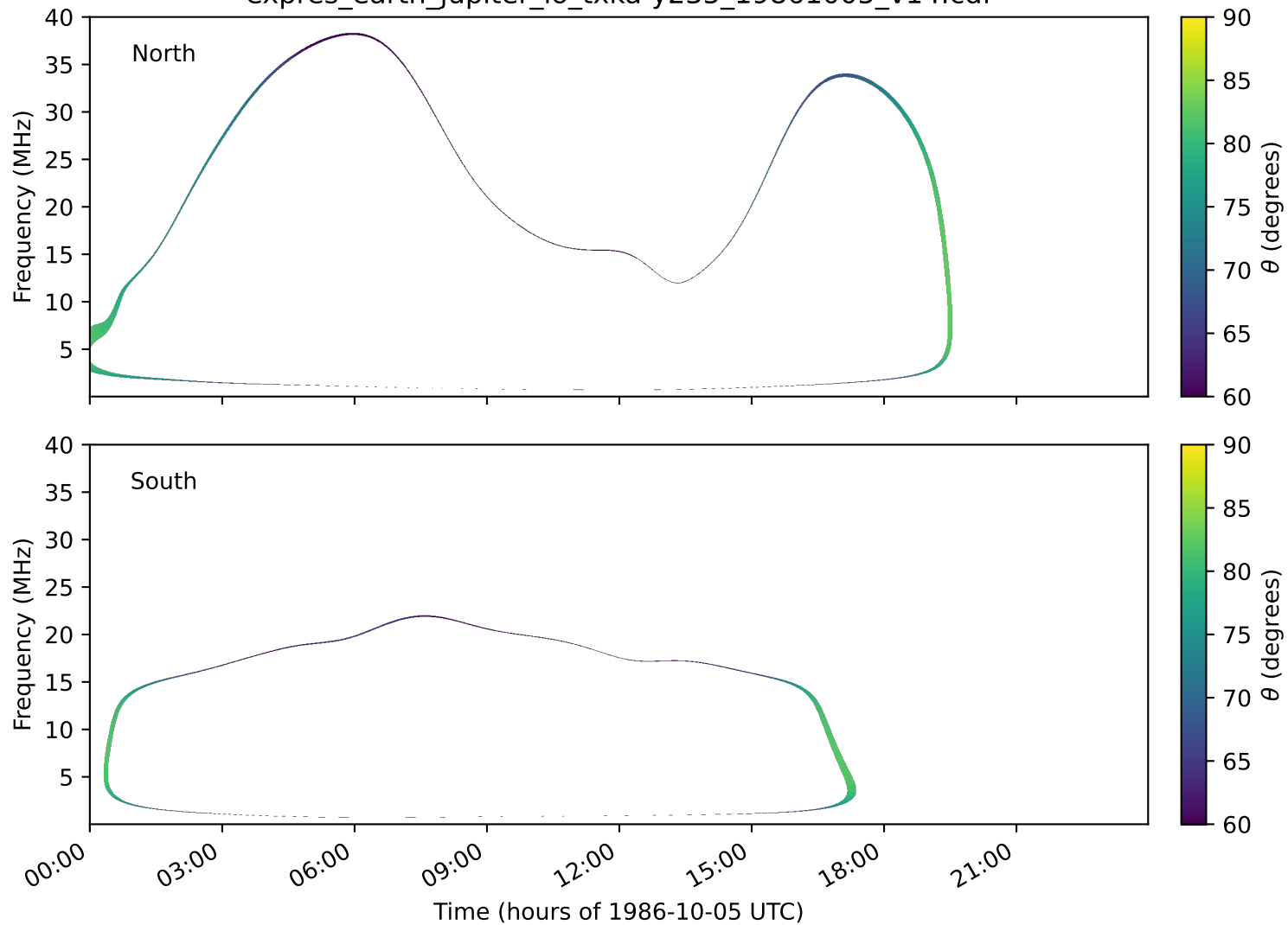
expres_earth_jupiter_io_txka-y235_19861005_v14.cdf
