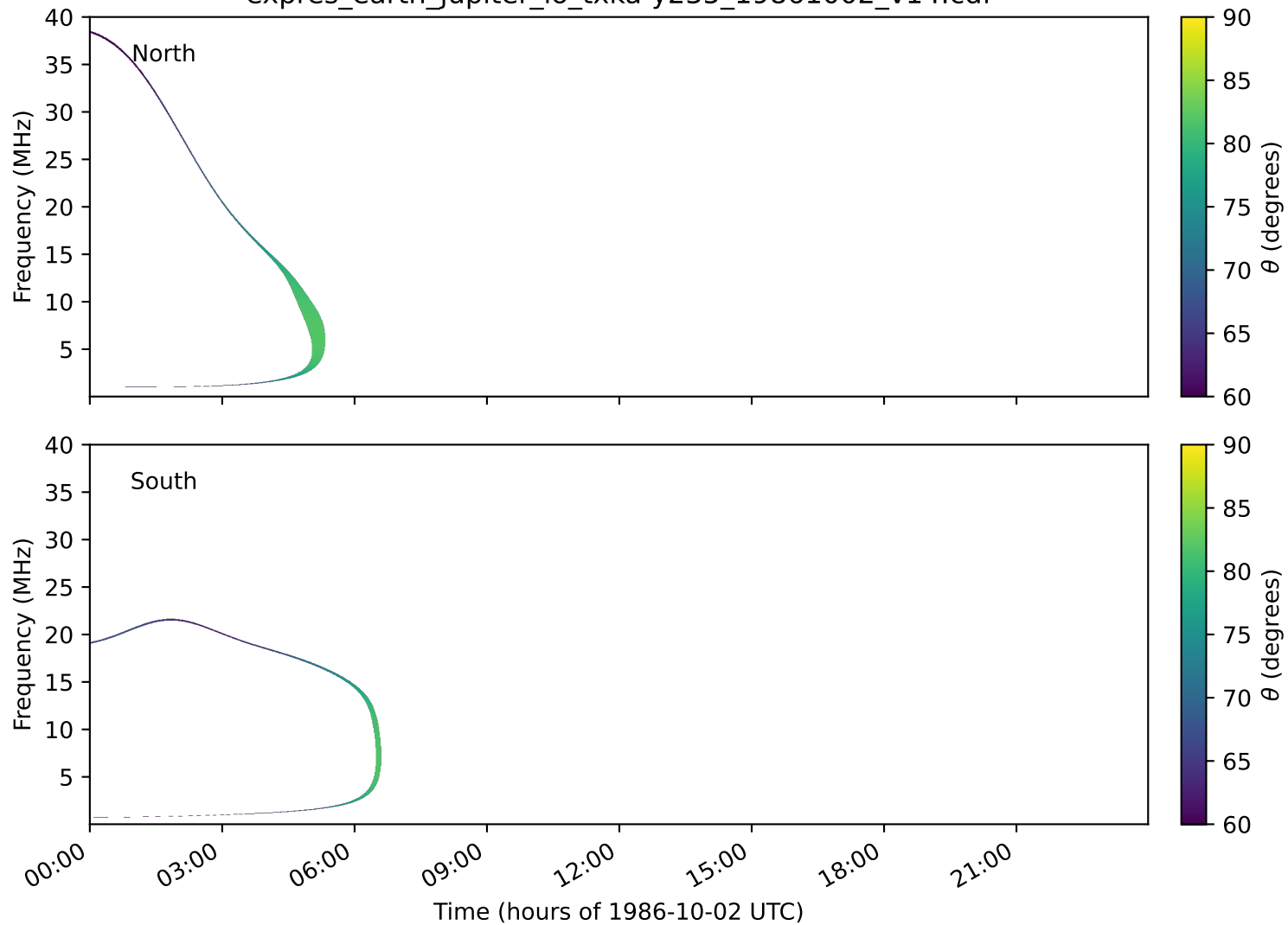
expres_earth_jupiter_io_txka-y235_19861002_v14.cdf
