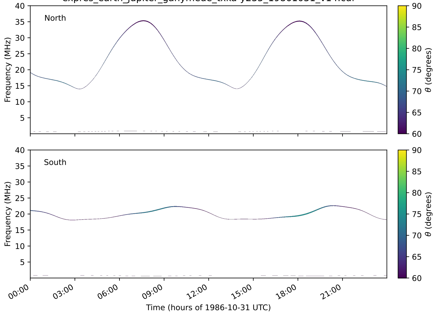
expres_earth_jupiter_ganymede_txka-y235_19861031_v14.cdf
