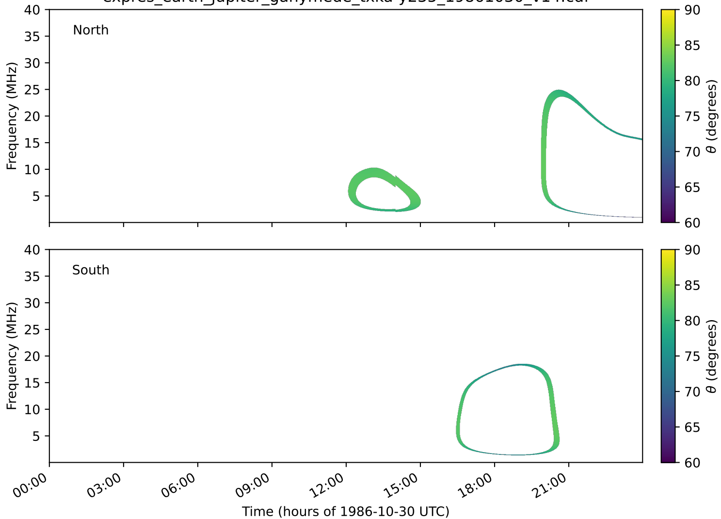
expres_earth_jupiter_ganymede_txka-y235_19861030_v14.cdf
