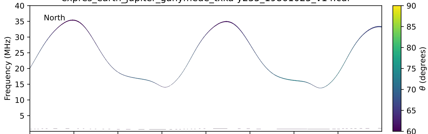
expres_earth_jupiter_ganymede_txka-y235_19861025_v14.cdf
