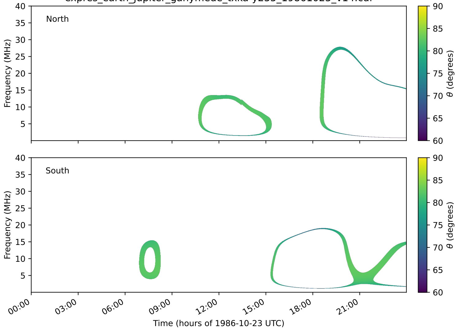
expres_earth_jupiter_ganymede_txka-y235_19861023_v14.cdf
