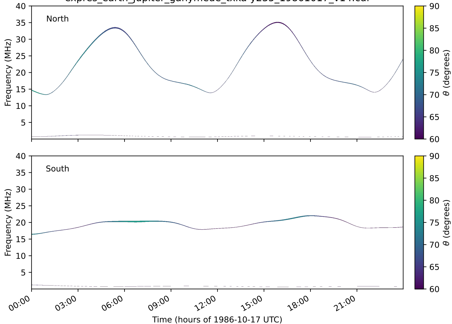
expres_earth_jupiter_ganymede_txka-y235_19861017_v14.cdf
