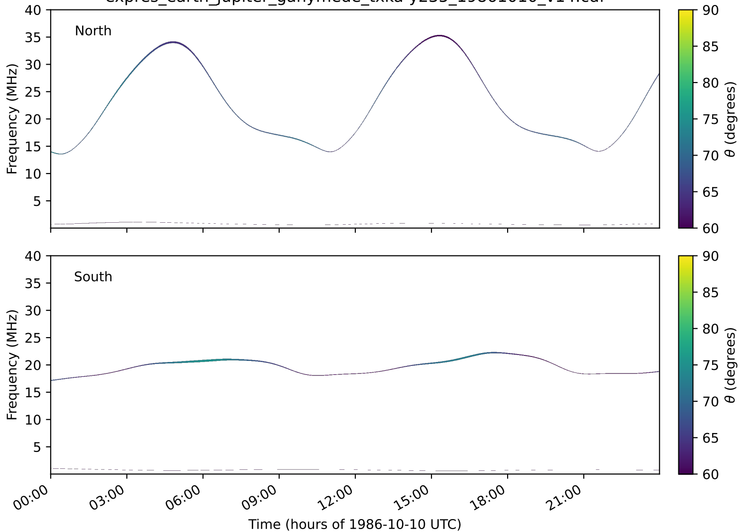
expres_earth_jupiter_ganymede_txka-y235_19861010_v14.cdf
