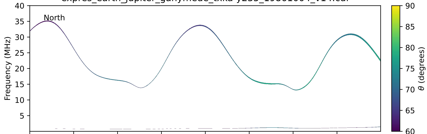
expres_earth_jupiter_ganymede_txka-y235_19861004_v14.cdf
