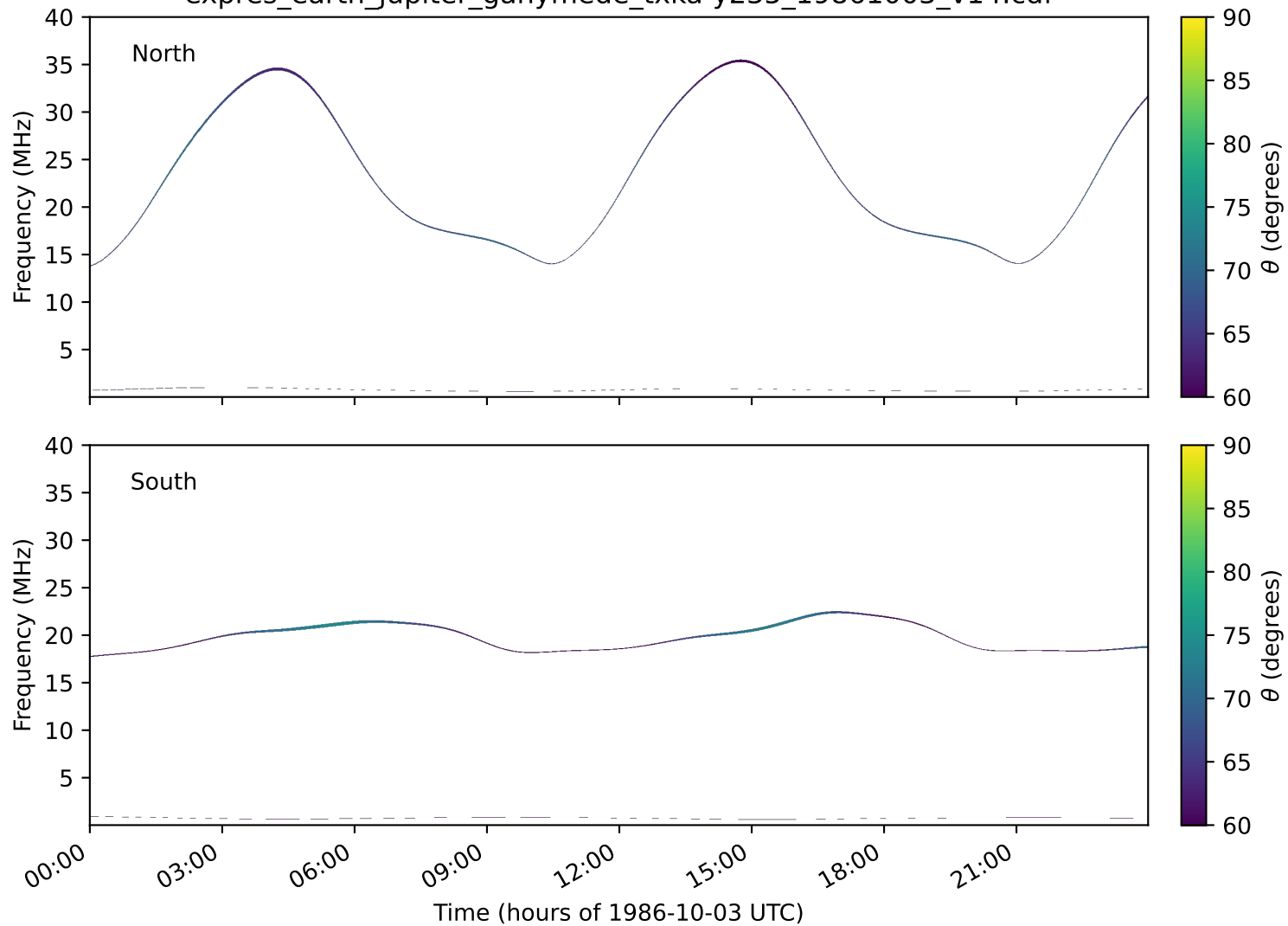
expres_earth_jupiter_ganymede_txka-y235_19861003_v14.cdf
