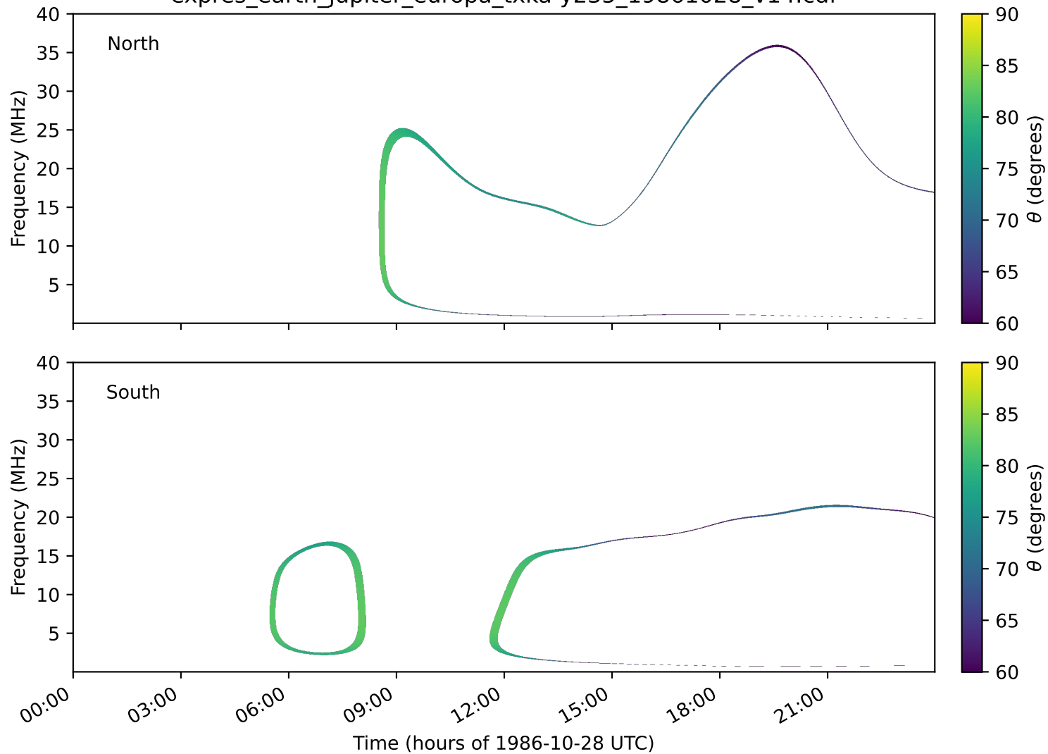
expres_earth_jupiter_europa_txka-y235_19861028_v14.cdf
