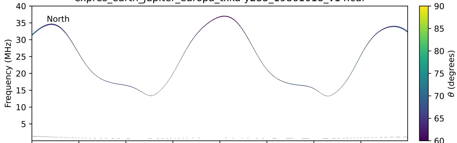
expres_earth_jupiter_europa_txka-y235_19861018_v14.cdf
