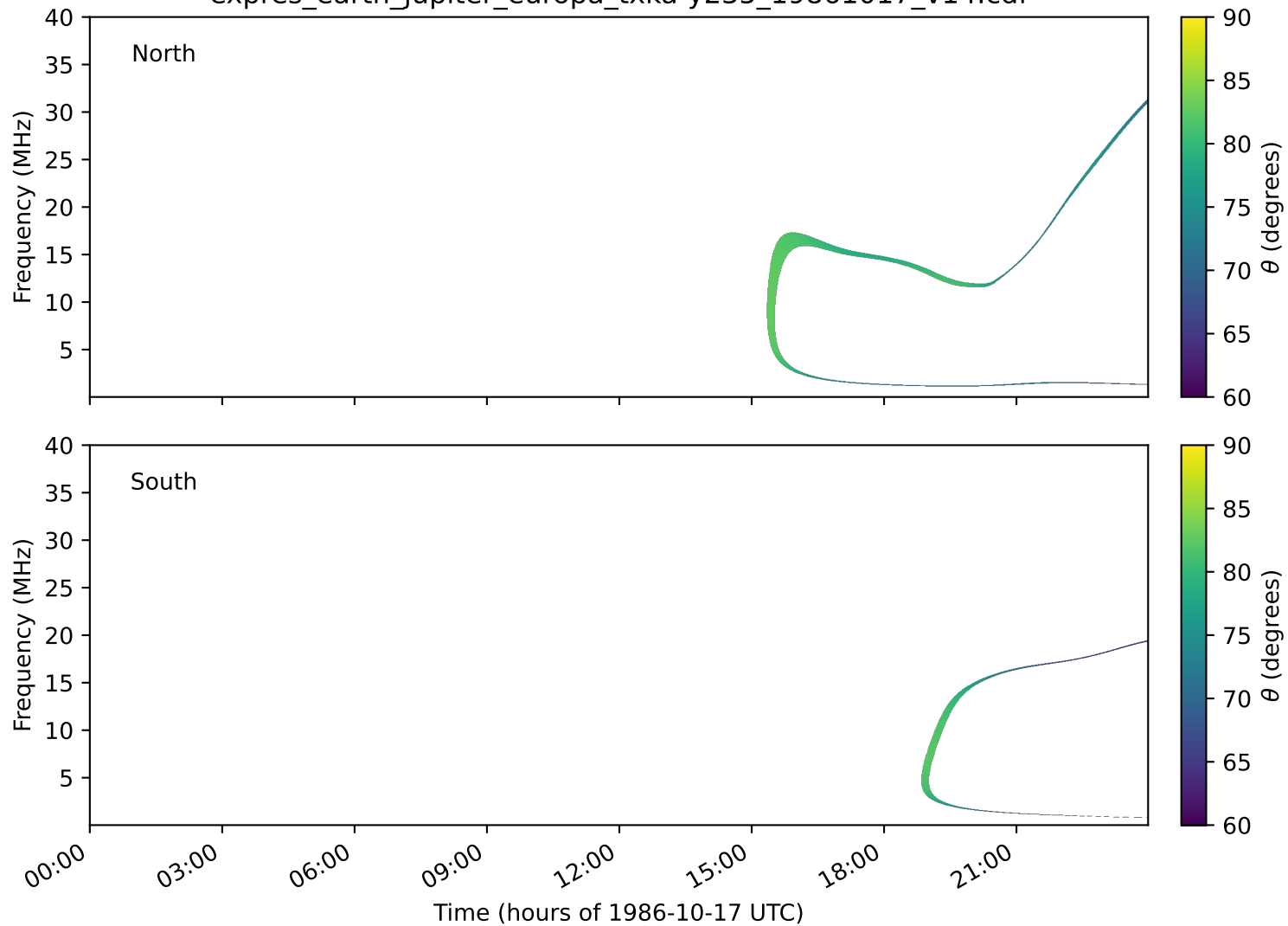
expres_earth_jupiter_europa_txka-y235_19861017_v14.cdf
