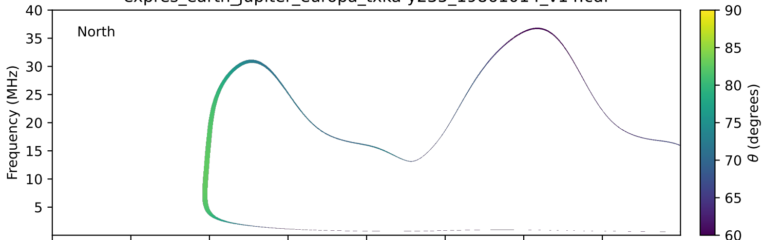
expres_earth_jupiter_europa_txka-y235_19861014_v14.cdf
