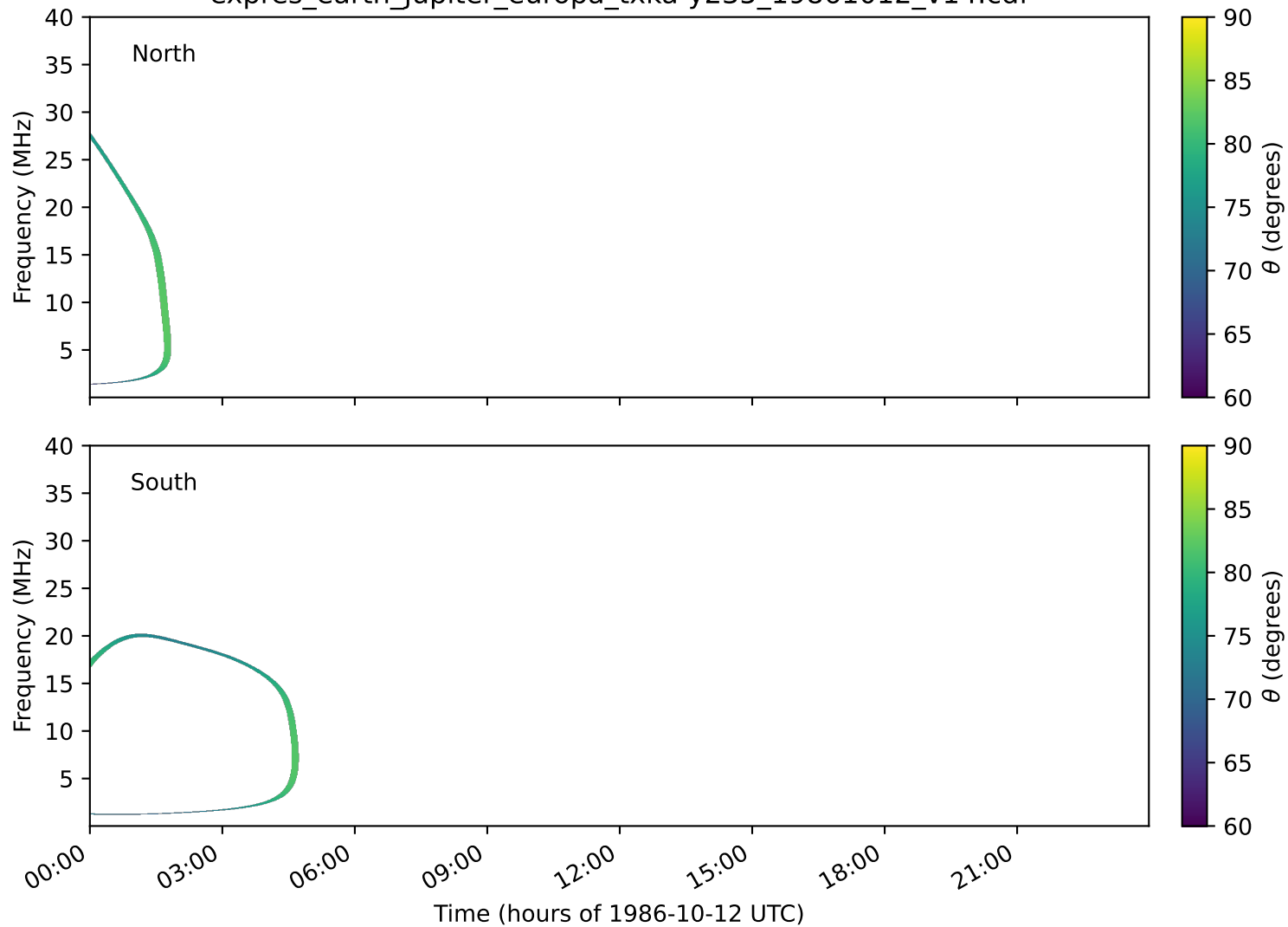
expres_earth_jupiter_europa_txka-y235_19861012_v14.cdf
