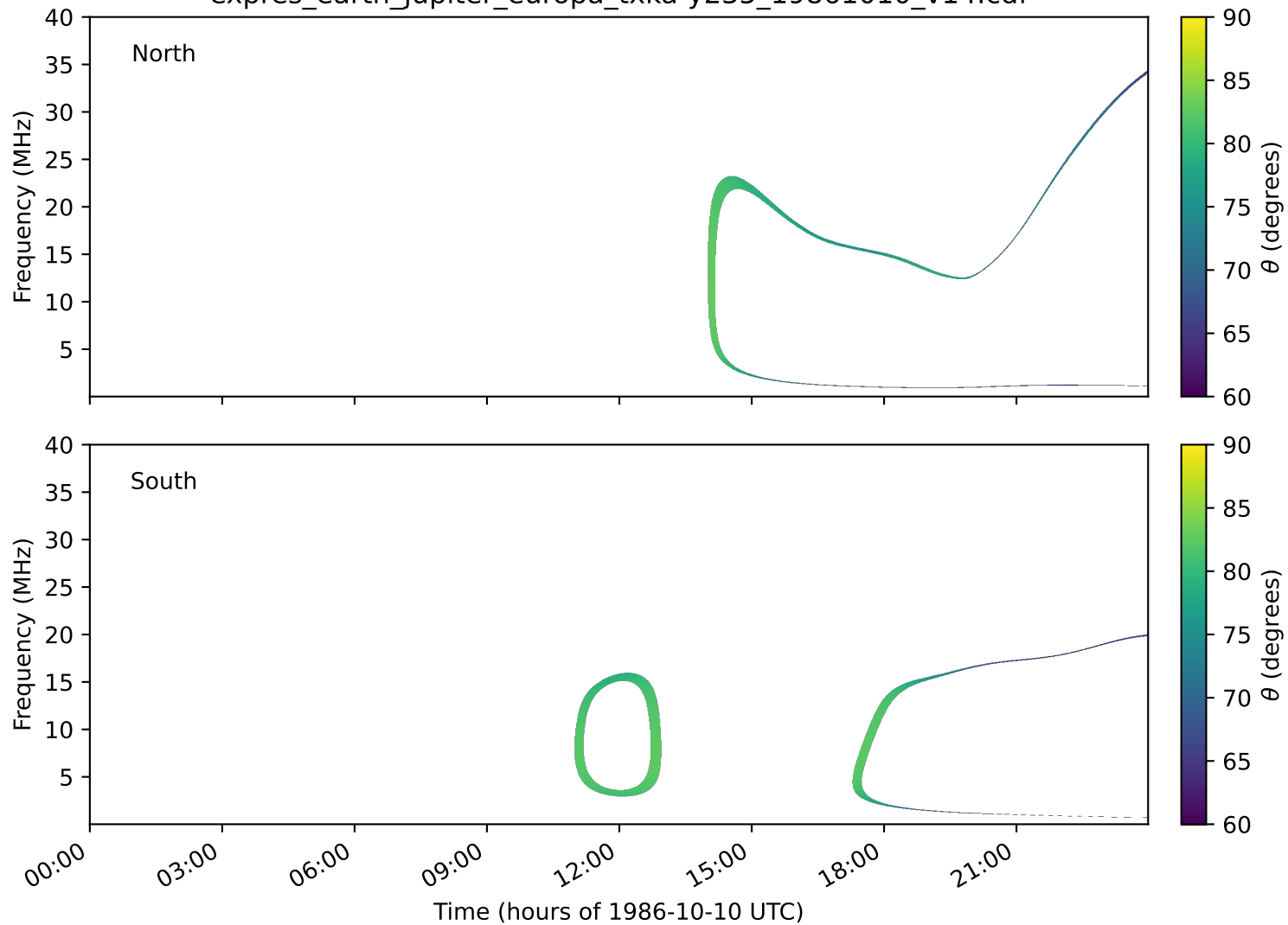
expres_earth_jupiter_europa_txka-y235_19861010_v14.cdf
