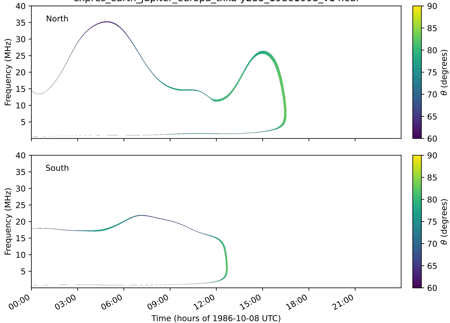
expres_earth_jupiter_europa_txka-y235_19861008_v14.cdf
