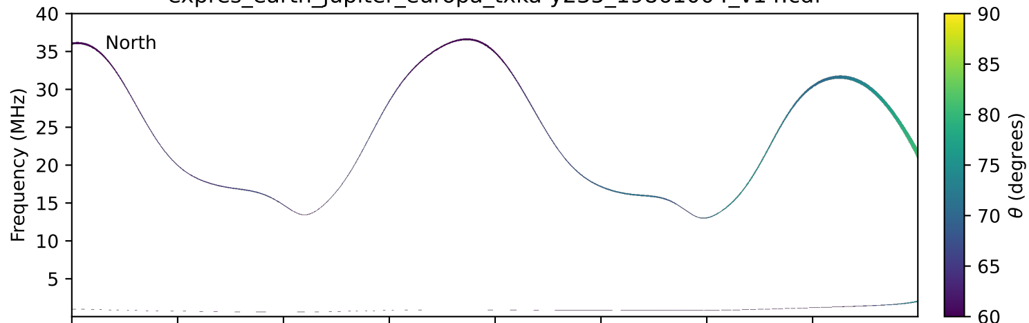
expres_earth_jupiter_europa_txka-y235_19861004_v14.cdf
