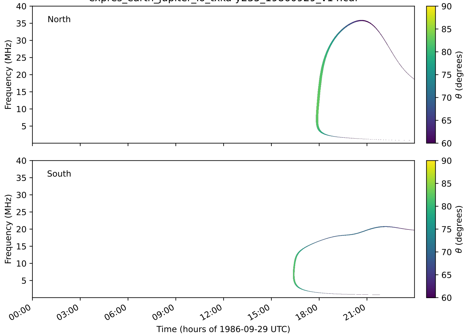
expres_earth_jupiter_io_txka-y235_19860929_v14.cdf
