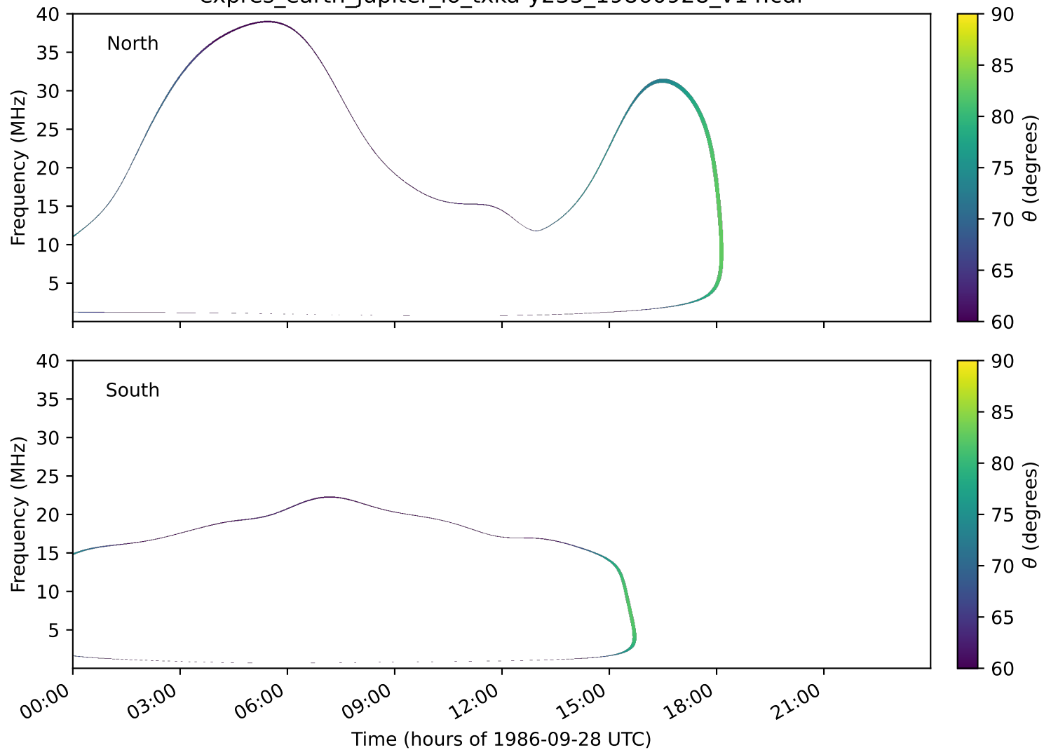
expres_earth_jupiter_io_txka-y235_19860928_v14.cdf
