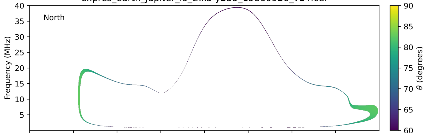
expres_earth_jupiter_io_txka-y235_19860926_v14.cdf
