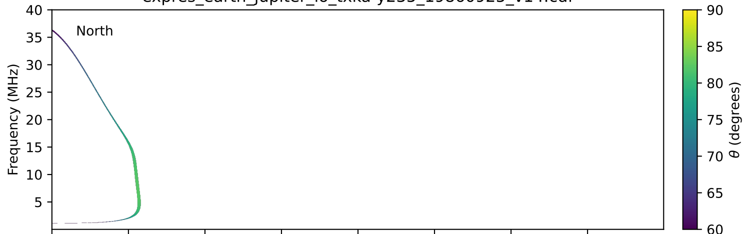
expres_earth_jupiter_io_txka-y235_19860925_v14.cdf
