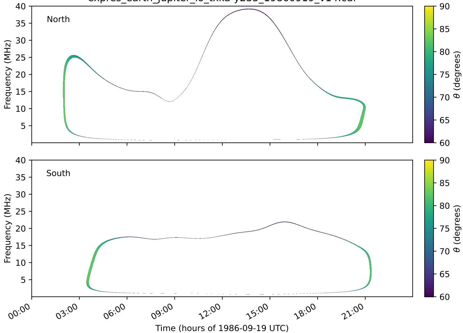
expres_earth_jupiter_io_txka-y235_19860919_v14.cdf
