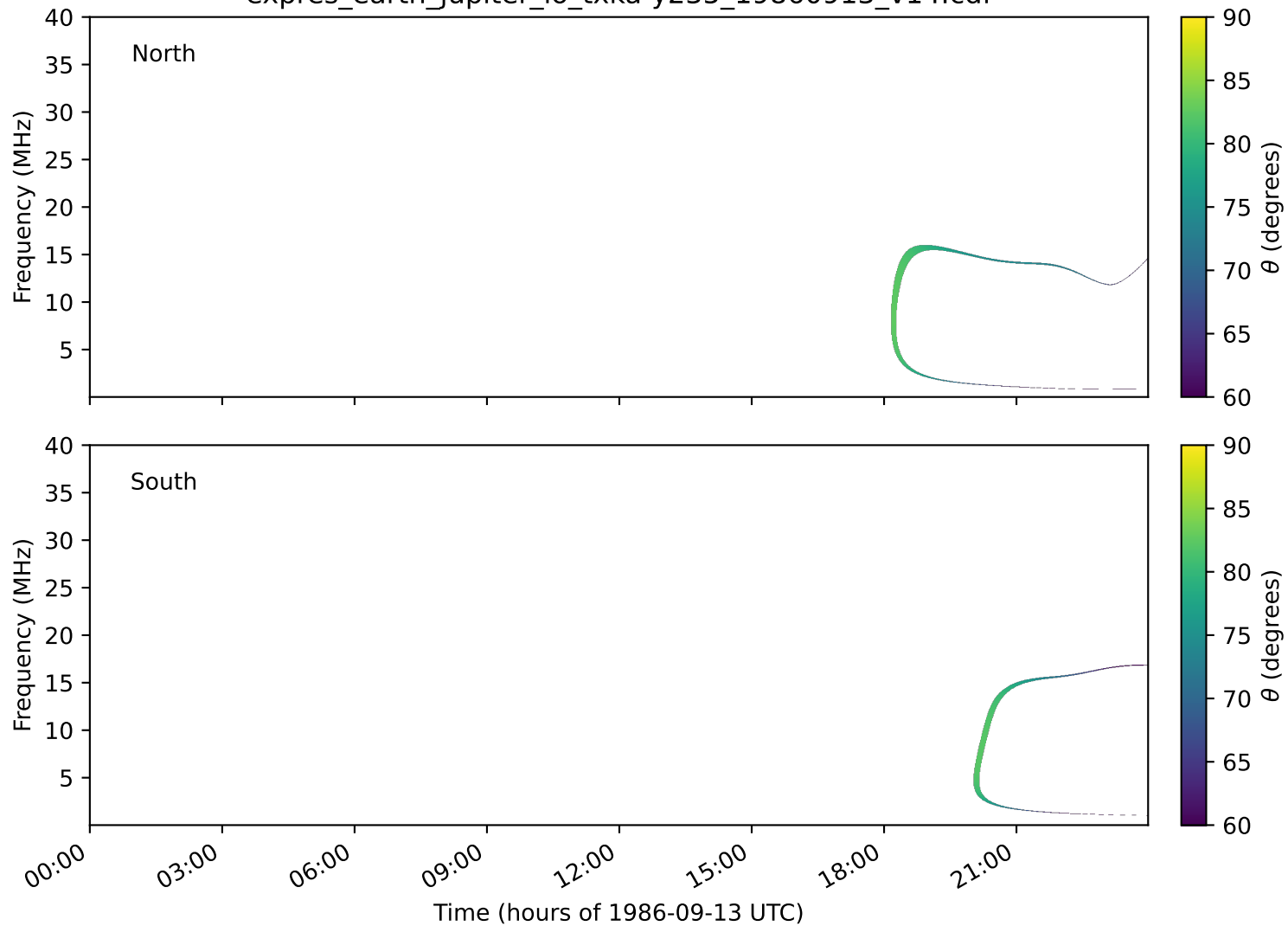
expres_earth_jupiter_io_txka-y235_19860913_v14.cdf
