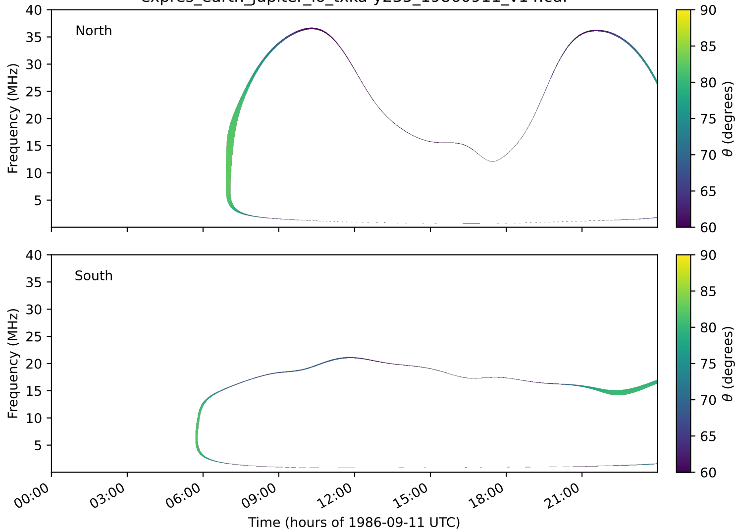
expres_earth_jupiter_io_txka-y235_19860911_v14.cdf
