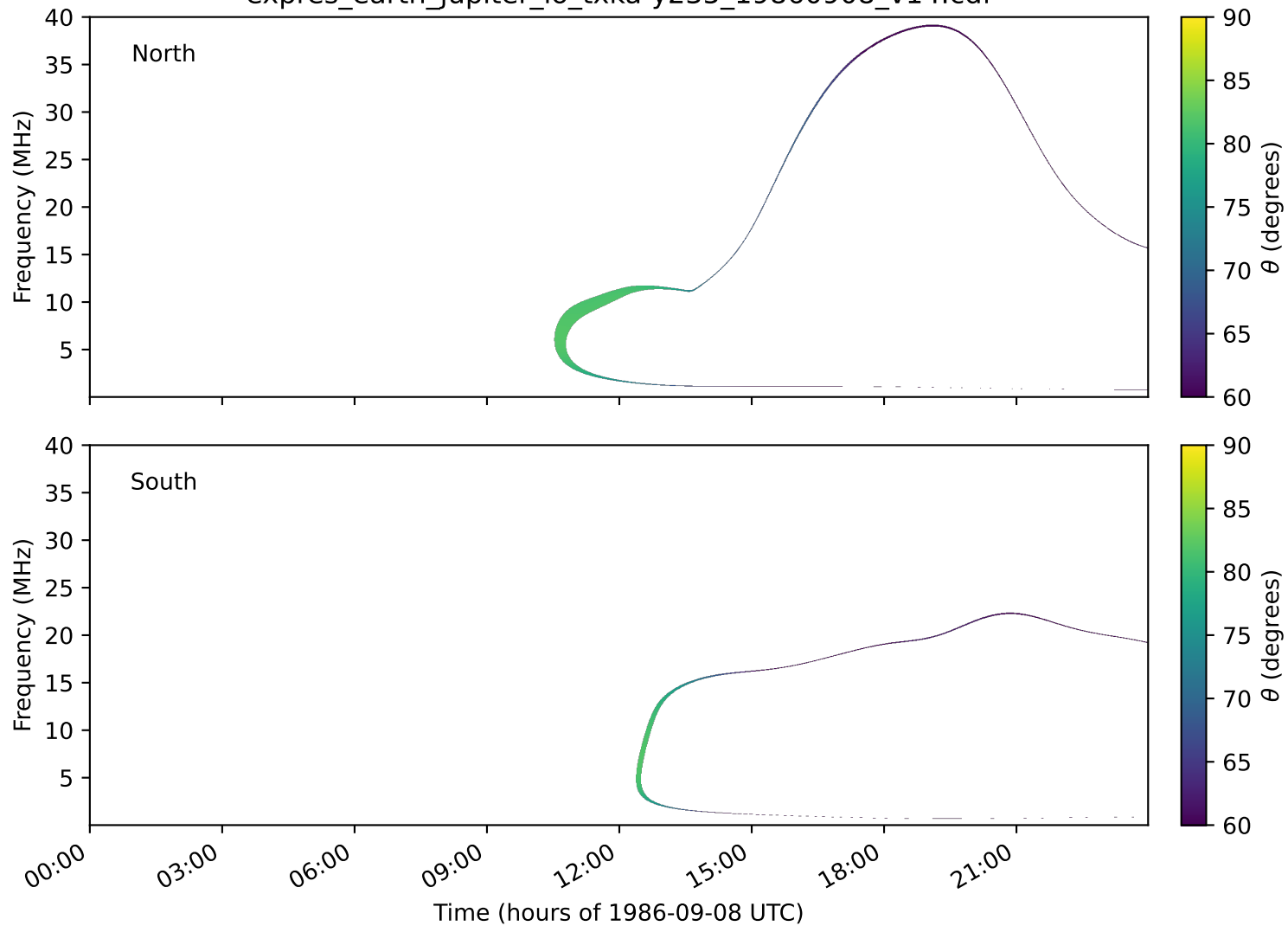
expres_earth_jupiter_io_txka-y235_19860908_v14.cdf
