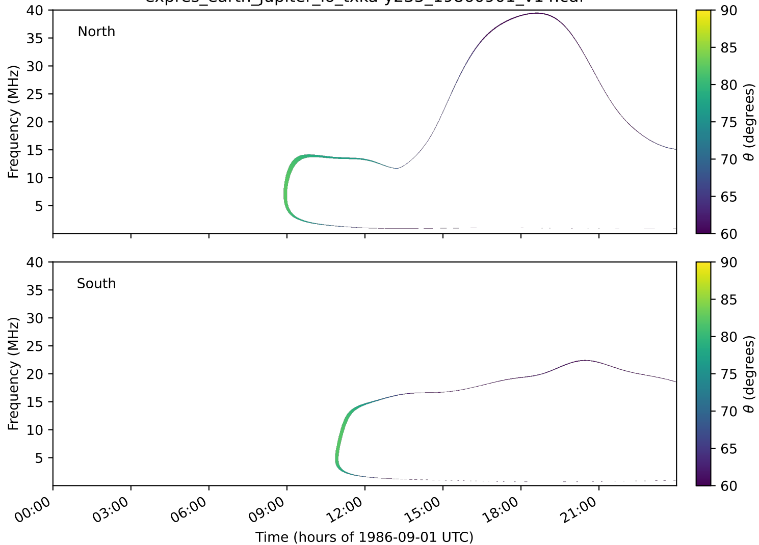
expres_earth_jupiter_io_txka-y235_19860901_v14.cdf
