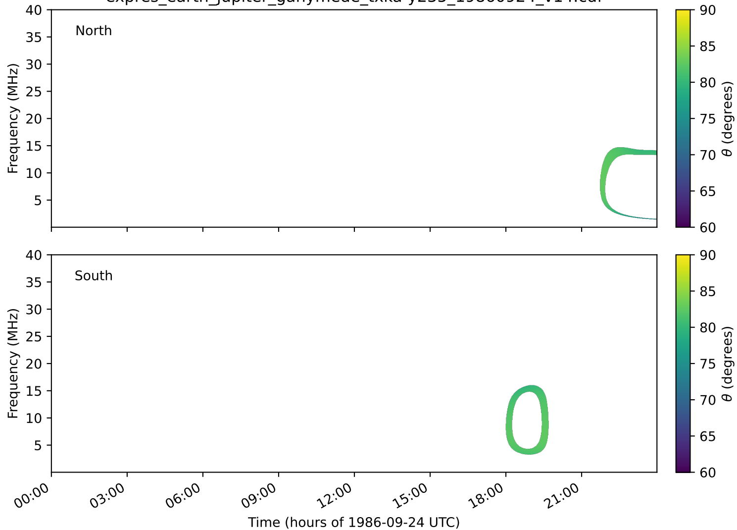
expres_earth_jupiter_ganymede_txka-y235_19860924_v14.cdf
