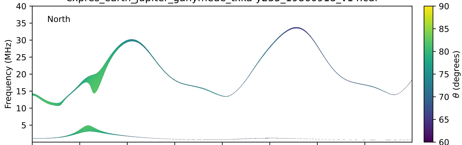
expres_earth_jupiter_ganymede_txka-y235_19860918_v14.cdf
