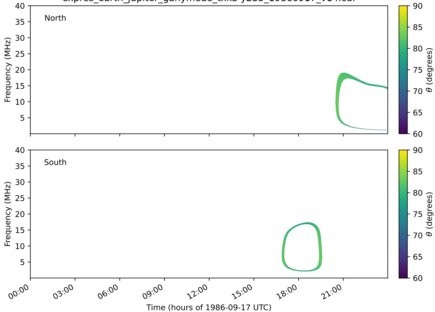
expres_earth_jupiter_ganymede_txka-y235_19860917_v14.cdf
