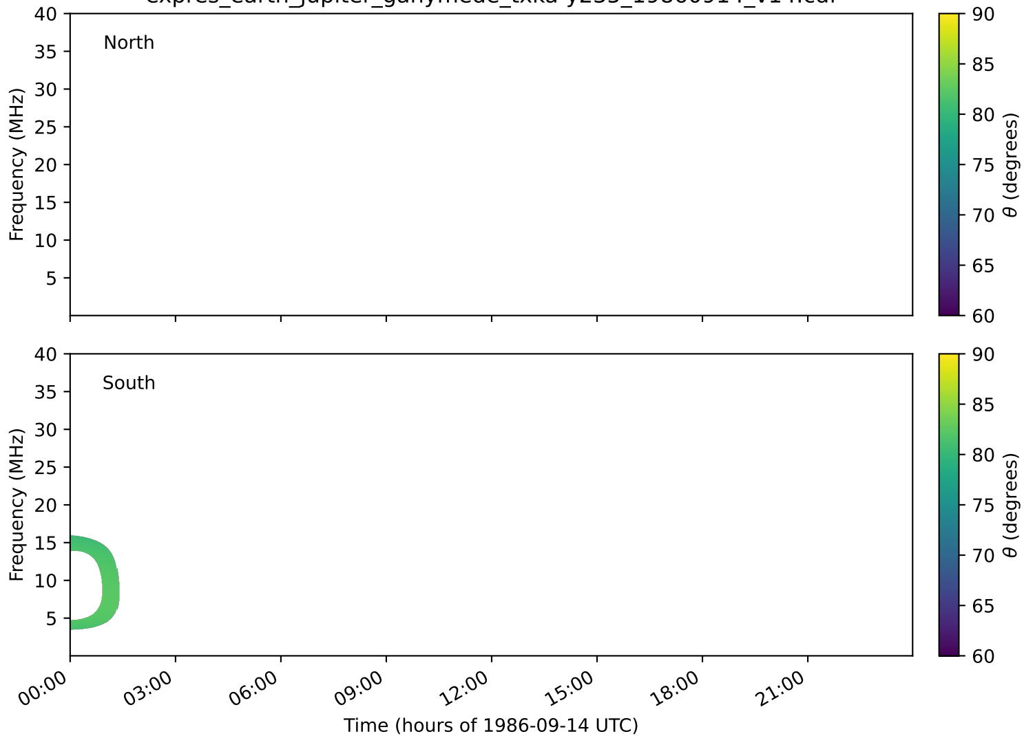
expres_earth_jupiter_ganymede_txka-y235_19860914_v14.cdf
