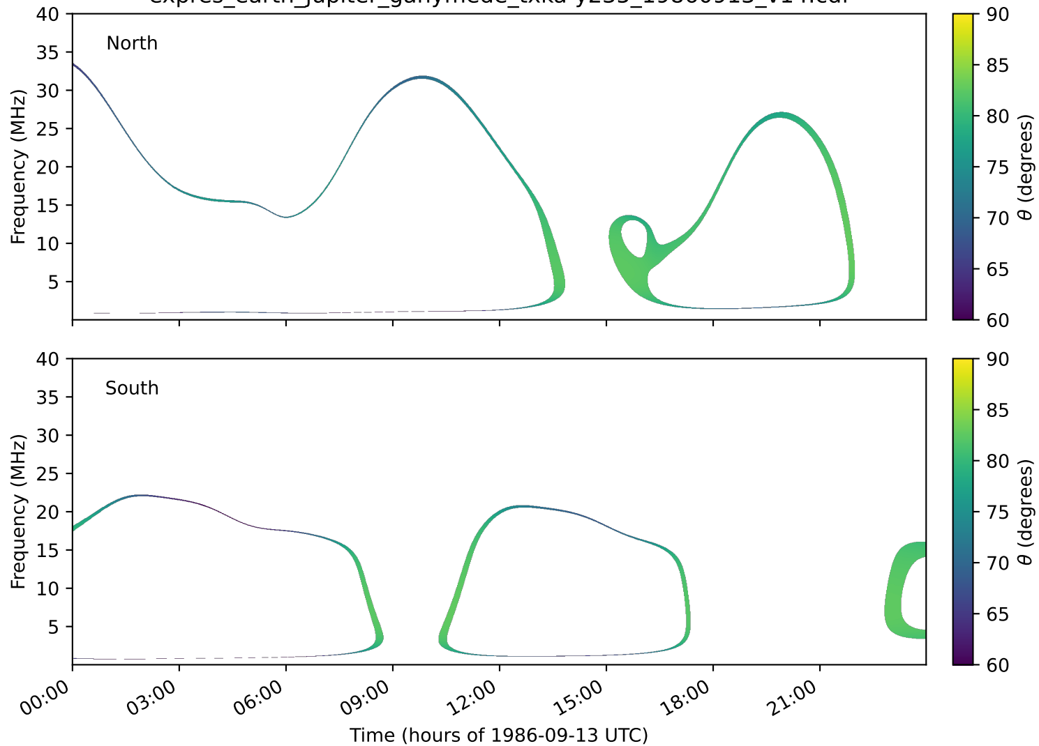
expres_earth_jupiter_ganymede_txka-y235_19860913_v14.cdf
