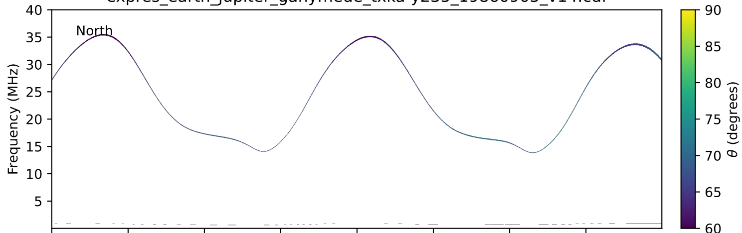
expres_earth_jupiter_ganymede_txka-y235_19860905_v14.cdf
