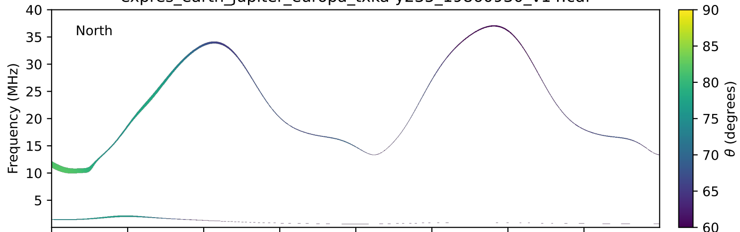
expres_earth_jupiter_europa_txka-y235_19860930_v14.cdf
