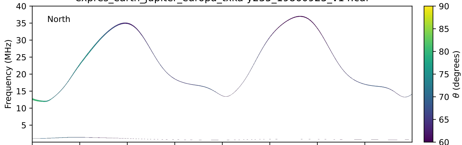
expres_earth_jupiter_europa_txka-y235_19860923_v14.cdf
