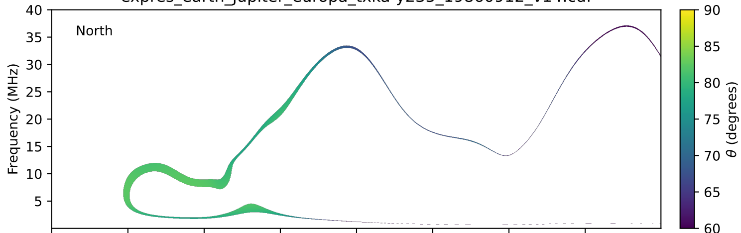
expres_earth_jupiter_europa_txka-y235_19860912_v14.cdf
