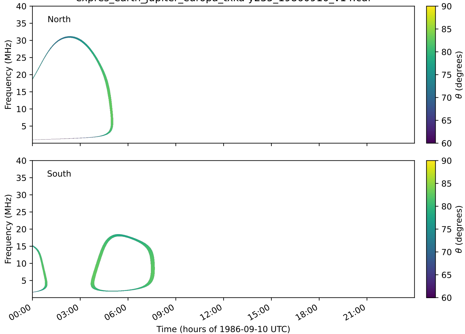
expres_earth_jupiter_europa_txka-y235_19860910_v14.cdf
