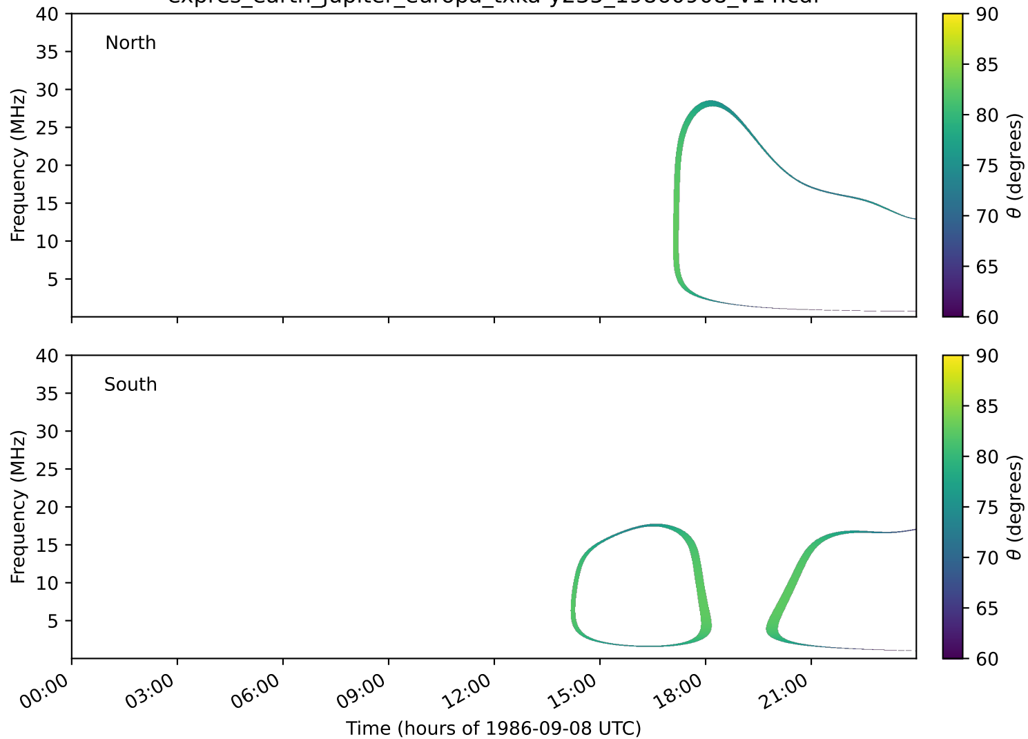
expres_earth_jupiter_europa_txka-y235_19860908_v14.cdf
