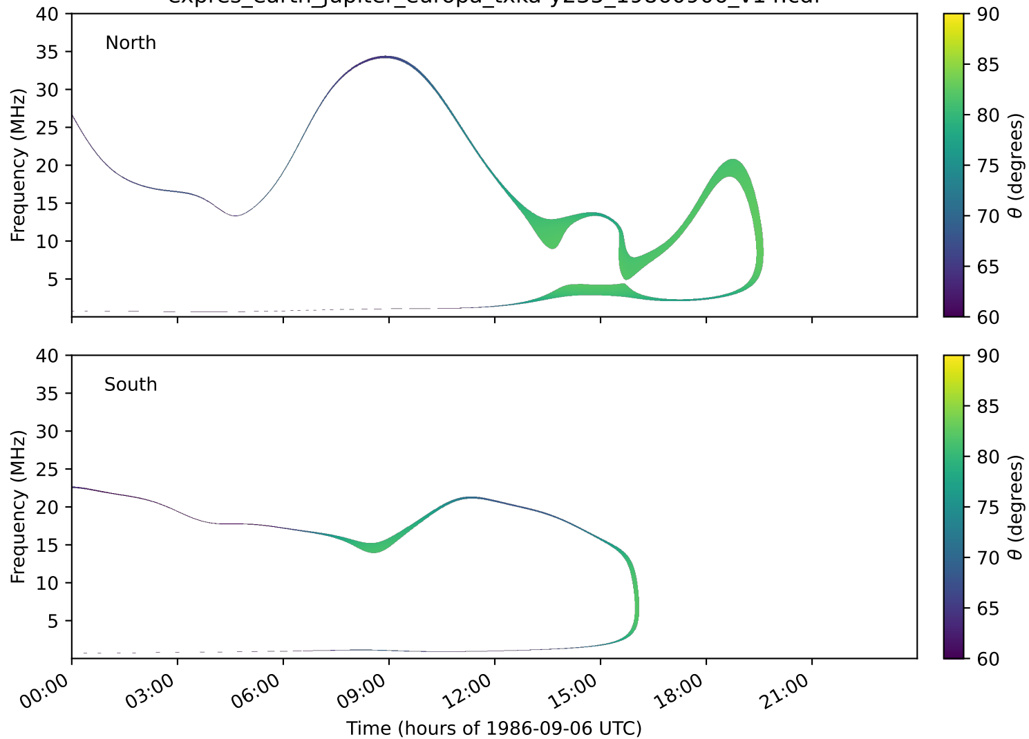
expres_earth_jupiter_europa_txka-y235_19860906_v14.cdf
