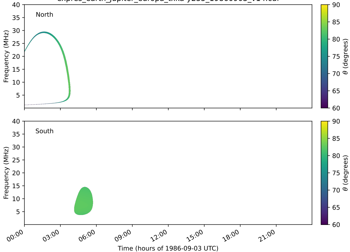
expres_earth_jupiter_europa_txka-y235_19860903_v14.cdf
