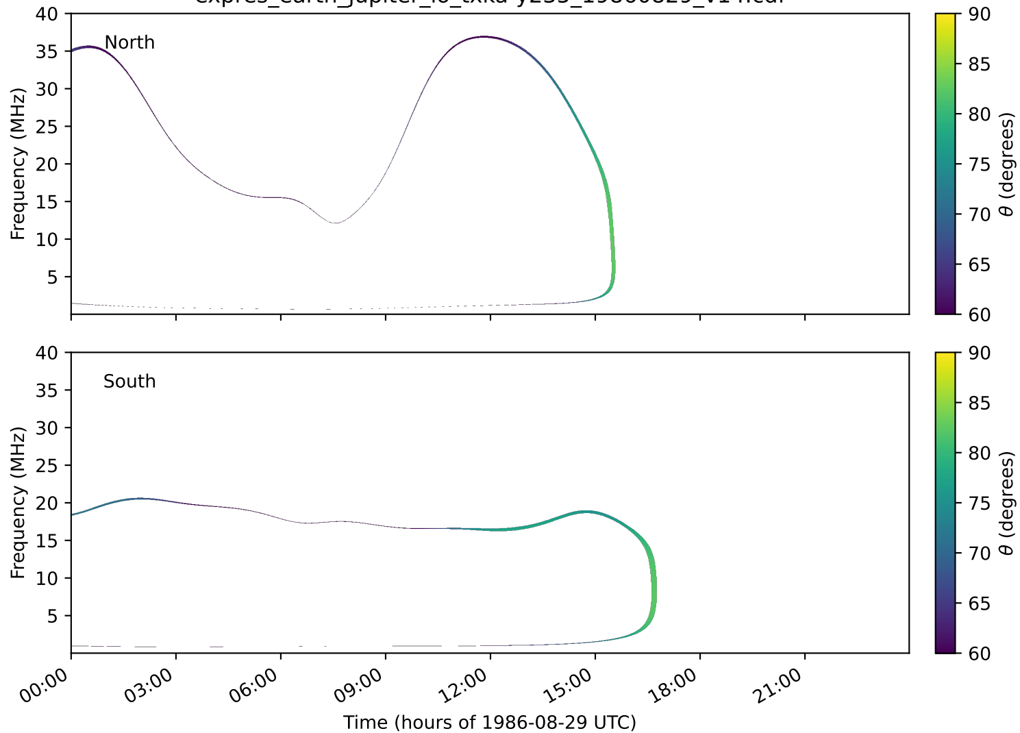
expres_earth_jupiter_io_txka-y235_19860829_v14.cdf
