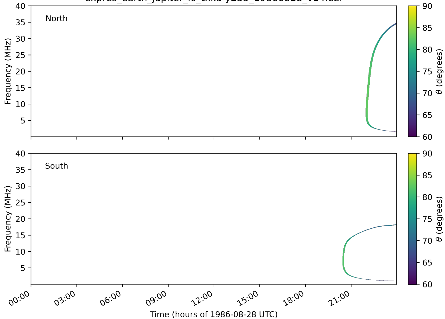
expres_earth_jupiter_io_txka-y235_19860828_v14.cdf
