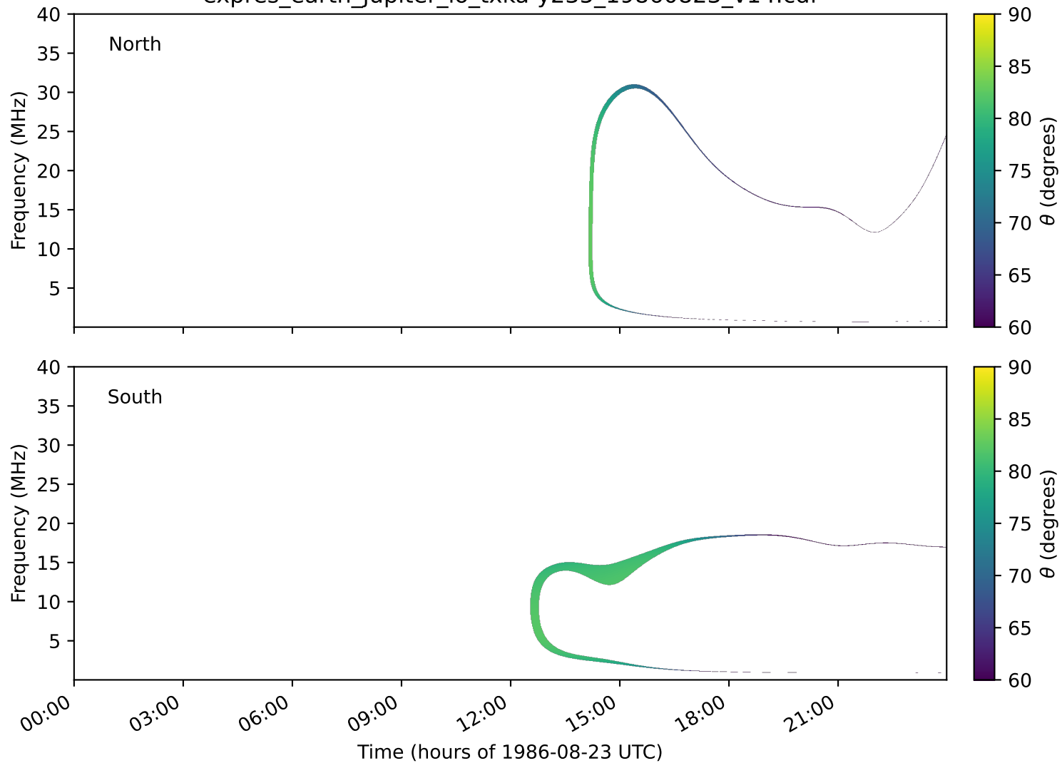
expres_earth_jupiter_io_txka-y235_19860823_v14.cdf
