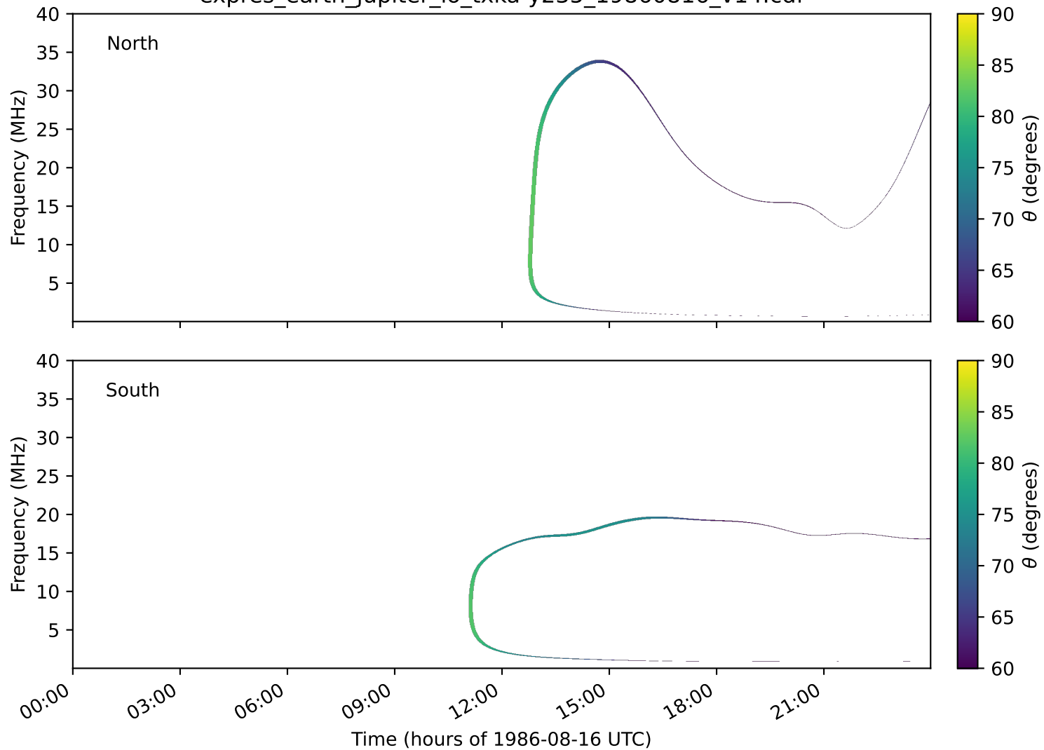
expres_earth_jupiter_io_txka-y235_19860816_v14.cdf
