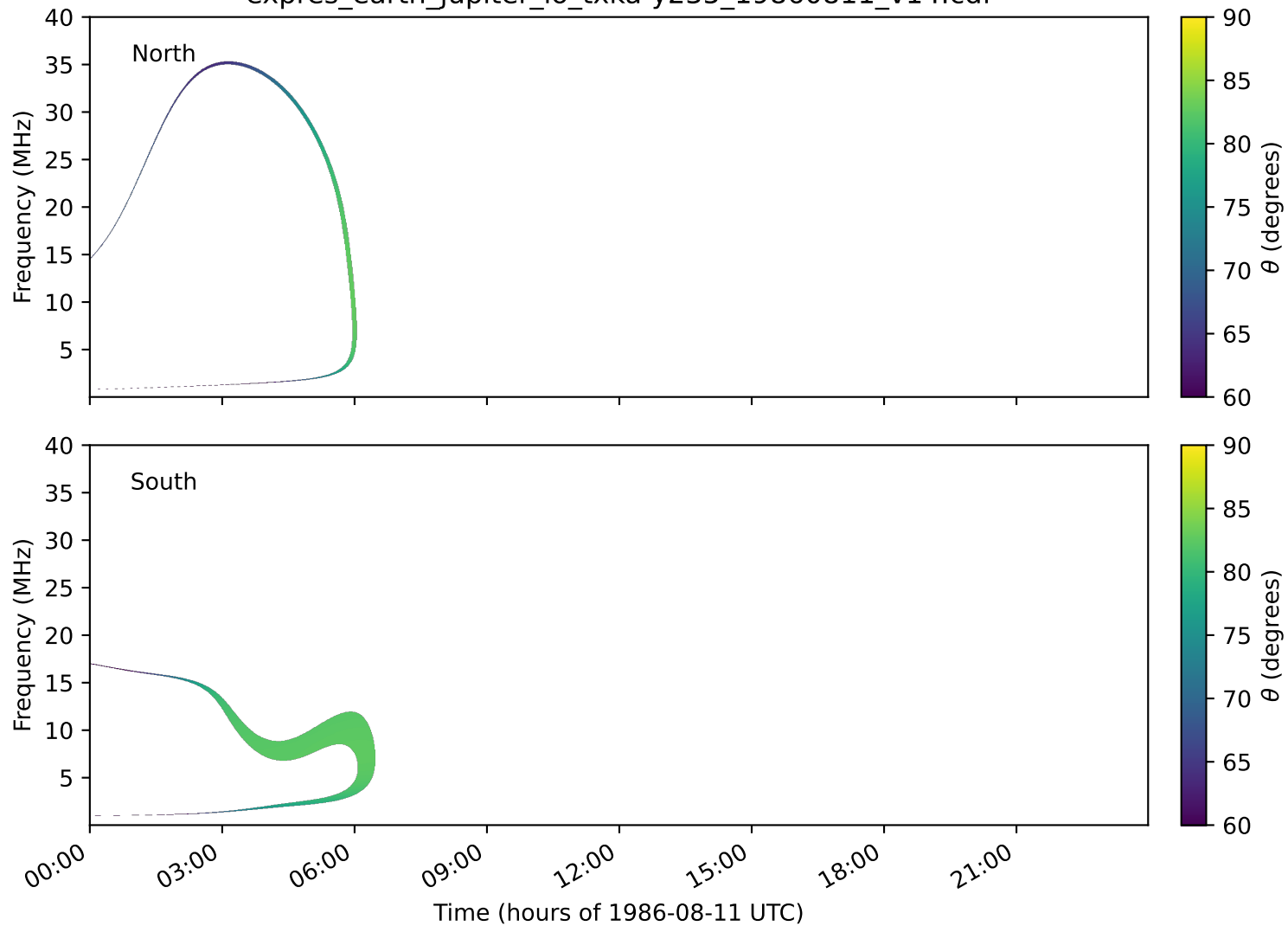
expres_earth_jupiter_io_txka-y235_19860811_v14.cdf
