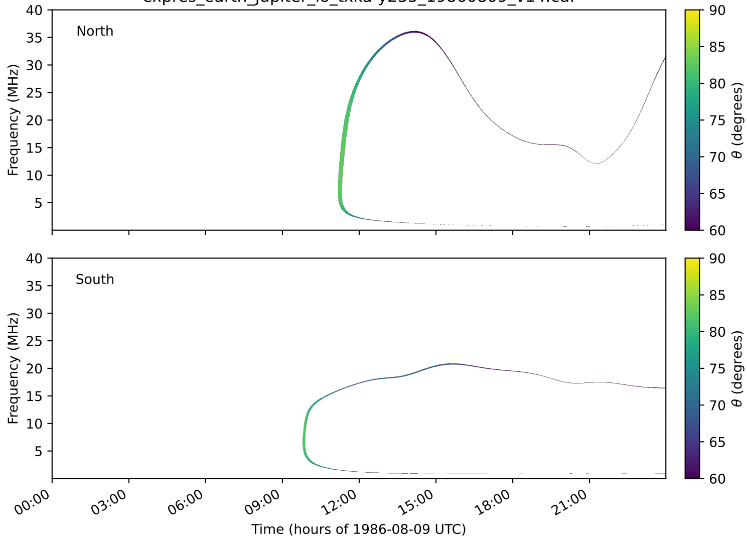
expres_earth_jupiter_io_txka-y235_19860809_v14.cdf
