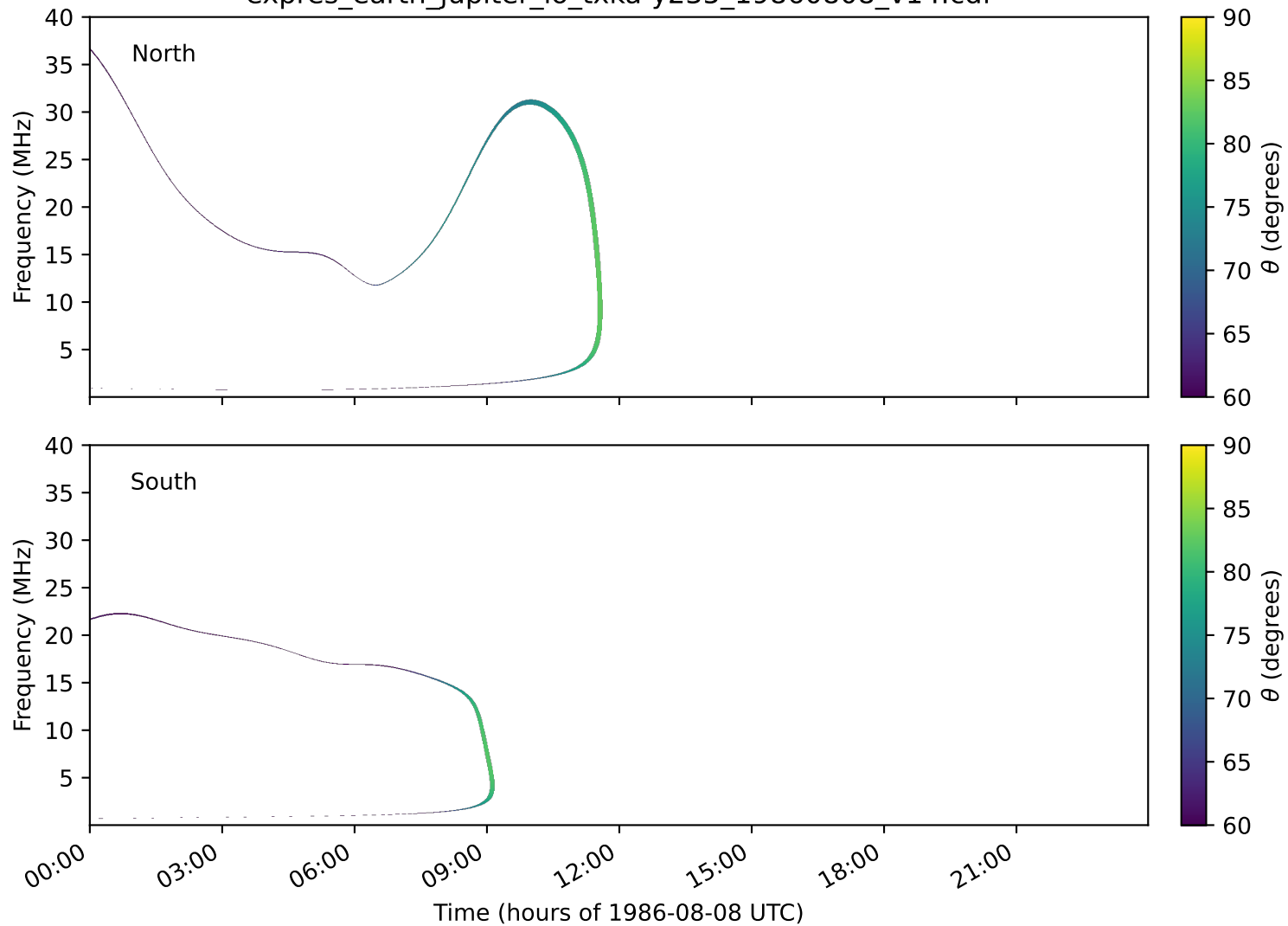
expres_earth_jupiter_io_txka-y235_19860808_v14.cdf
