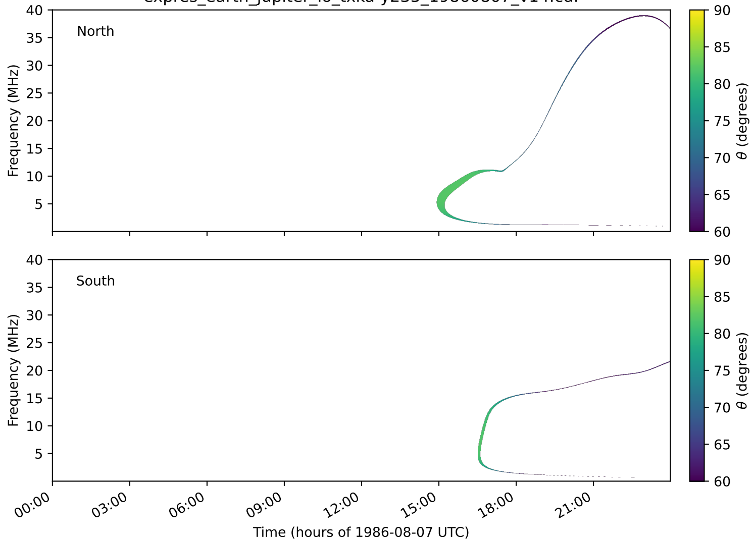
expres_earth_jupiter_io_txka-y235_19860807_v14.cdf
