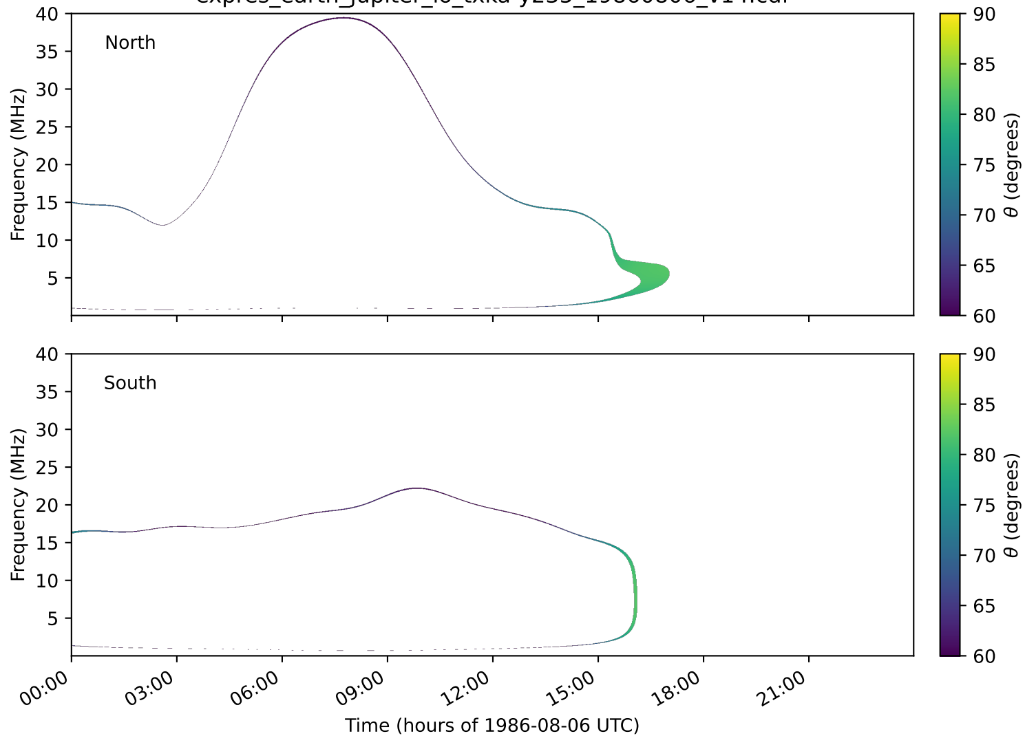
expres_earth_jupiter_io_txka-y235_19860806_v14.cdf
