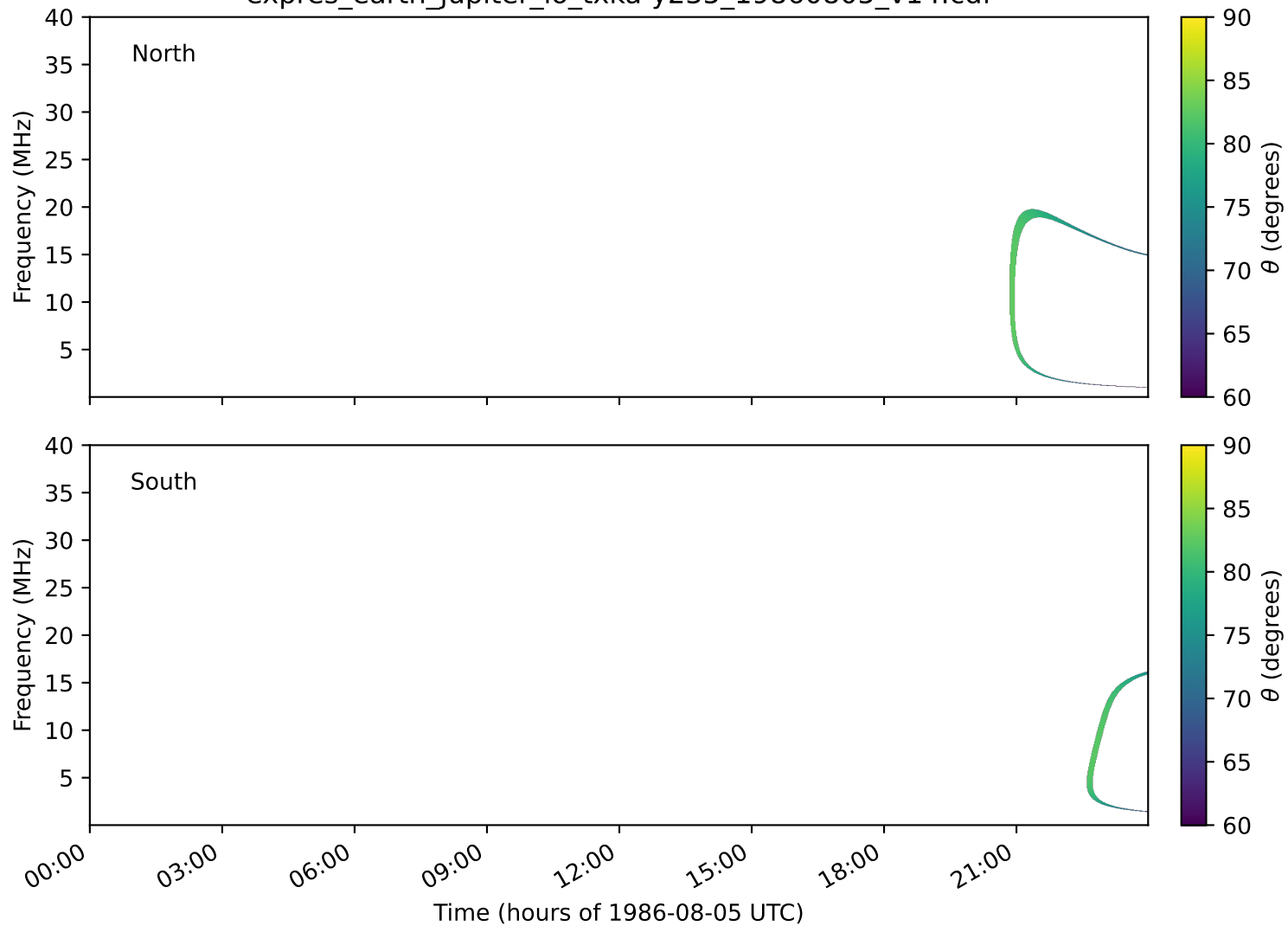
expres_earth_jupiter_io_txka-y235_19860805_v14.cdf
